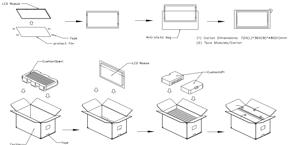
Figure. 7-1 Packing method
